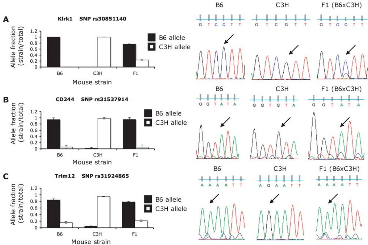
Figure 2. CNV mapping genes are regulated in cis . Allelic imbalance shows that CNV genes (A) Klrk1 , (B) CD244 and (C) Trim12 are regulated in cis . We used semi-quantitative sequence analysis in adipose cDNA from B6, C3H and B6×C3H F1 in cross 1, where we determined the ratio of the B6 and C3H alleles in the overall transcript levels of the F1 mice.
