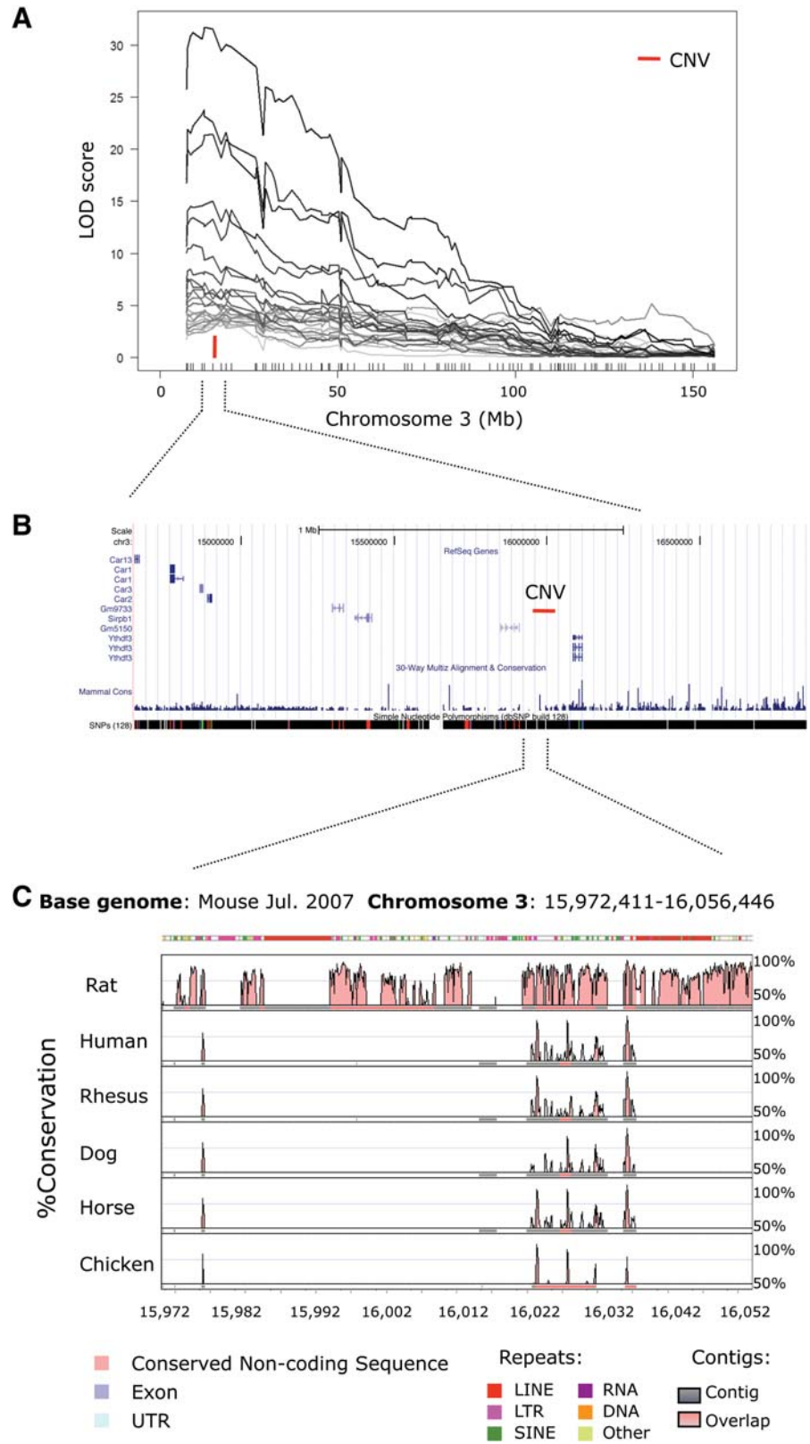
Figure 5. Mouse eQTL hotspot coincides with highly conserved non-coding sequences present in mouse CNVs. (A) A CNV in chromosome 3 coincides with the 95% confidence interval of 27 eQTL. Each curve represents an eQTL with LOD score >4.3 from female liver in cross 1. The red bar marks the position of the CNV. (B) The location of the CNV and neighboring genes in a 2 Mb window from the UCSC genome browser in Build37. Cross-species conservation for the CNV sequences is shown in (C), where the base mouse genome sequence (Build 37) is compared with the rat, human, rhesus macaque, dog, horse and chicken sequences. The degree of conservation is plotted on the y-axis as % identity over a 100 bp window. Highly conserved regions are highlighted under the curve, with a red color specifying non-coding sequences.
