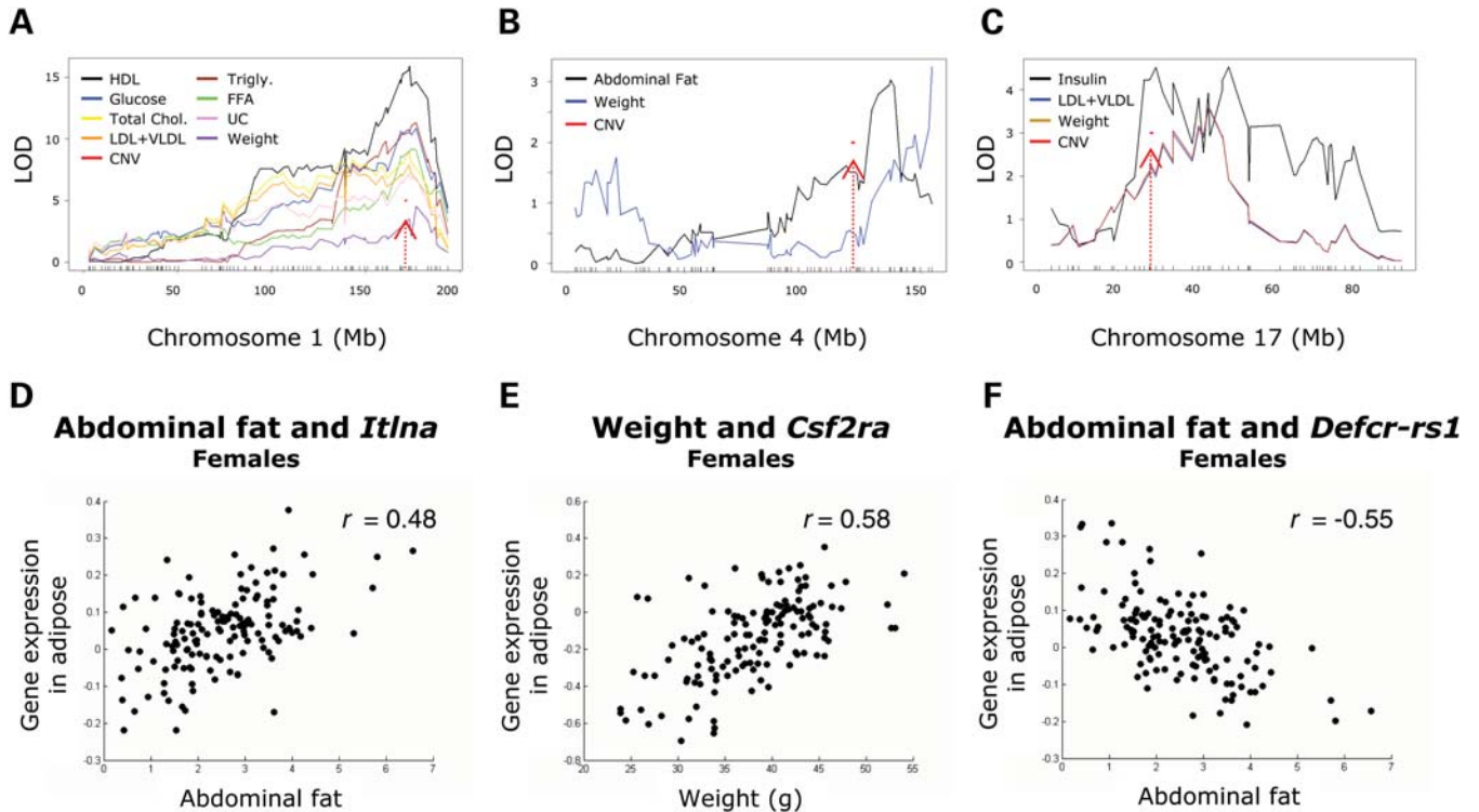
Figure 3. Impact of CNVs on metabolic traits. (A–C) Clinical QTL mapping reveals that CNVs overlap multiple cQTL in chromosomes 1, 4 and 17. (D–F) The expression levels of CNV genes are correlated with metabolic traits in B6×C3H F2 mice. The expression levels correspond to adipose tissue and F2 female mice. r Values correspond to the Pearson's correlation coefficient.
